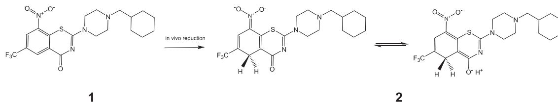
Fig. 1. Chemical structure of macozinone (PBTZ169) subjected in vivo to reduction into the Meisenheimer Complex H 2 PBTZ, shown as the two mesomeric forms in equilibrium.
